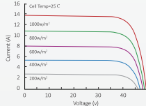
Current-Voltage Curve
