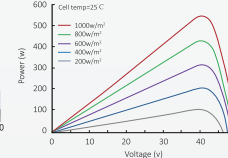
Power-Voltage Curve
